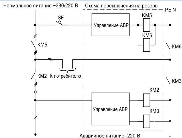
ПУ8255, ЯУ8255, ШУ8255
